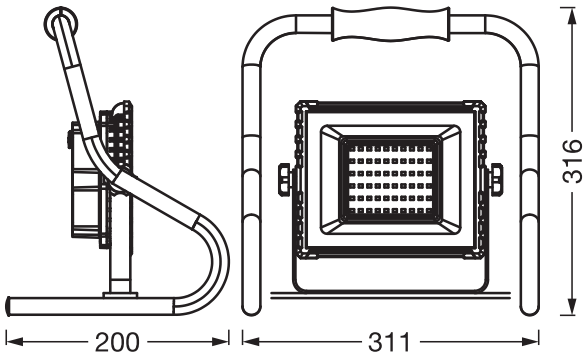
LED WORKLIGHT BATTERY 30W
