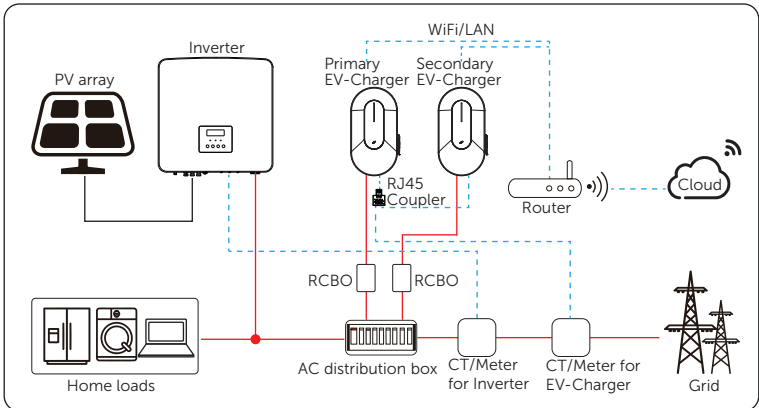
Figure 14-3 Parallel function - communication with CT/meter in Solar scene
