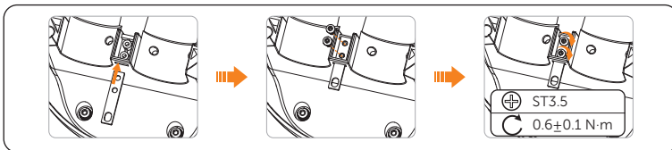
Figure 6-32 Install anti-theft accessory (b)
