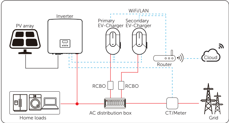
Figure 14-2 Parallel function - communication with inverter in Solar scene
